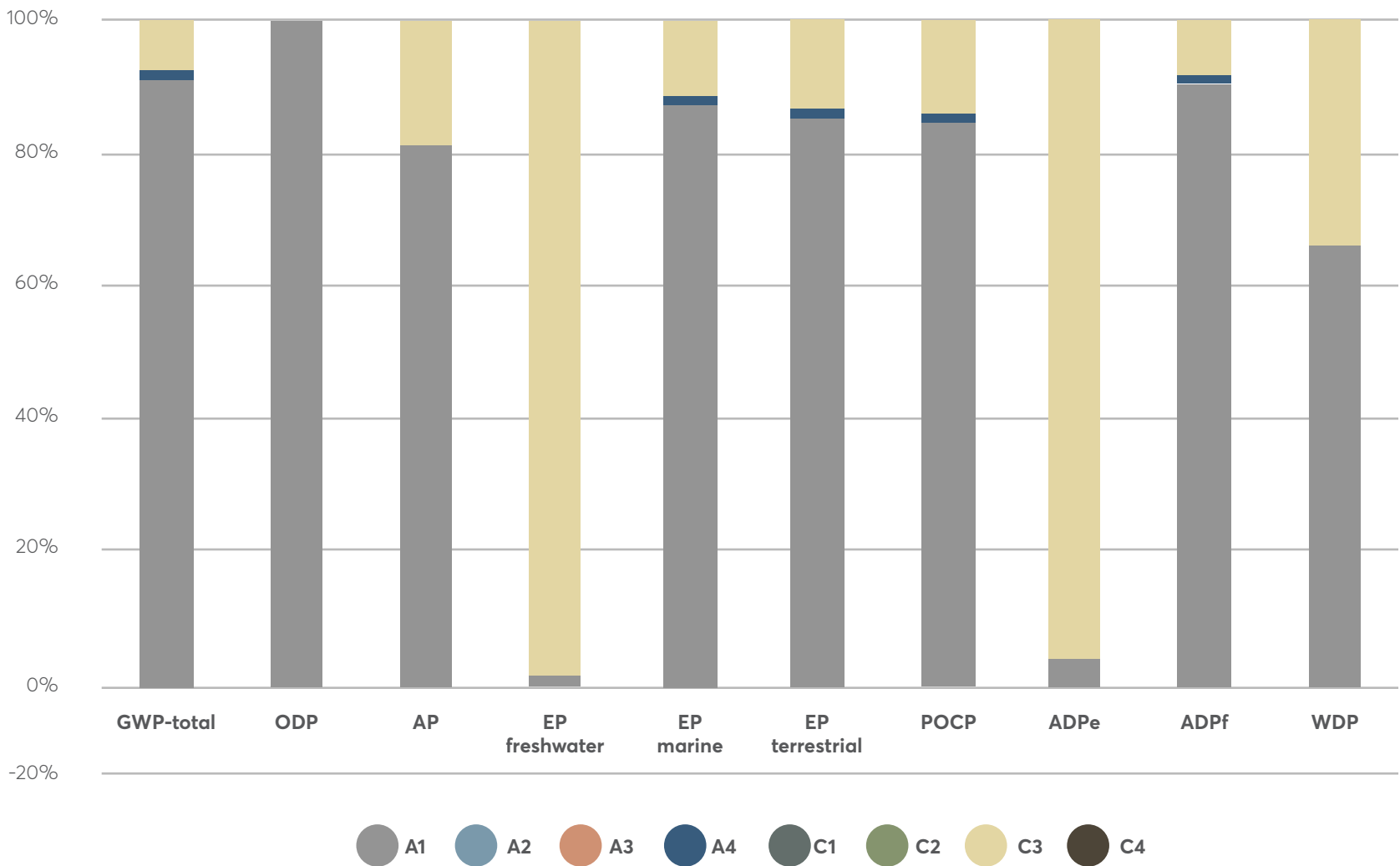
Characterized Results of Extruded Aluminium Profiles
